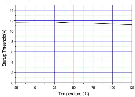
Figure 5. Start-Up Threshold vs Temperature
