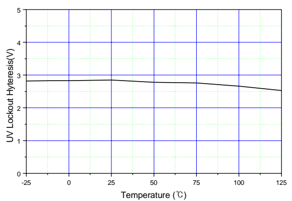
Figure 6. UV Lockout Hysteresis vs Temperature
